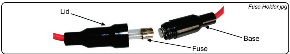
Figure 6: Fuse Holder
